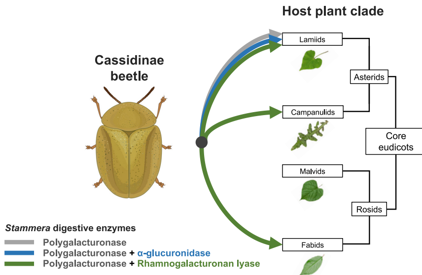
Figure 6. Cassidines Endowed with Stammera 's Polygalacturonase and Rhamnogalacturonan Lyase Have Radiated onto Host Plants Spanning a Wide Phylogenetic Range
